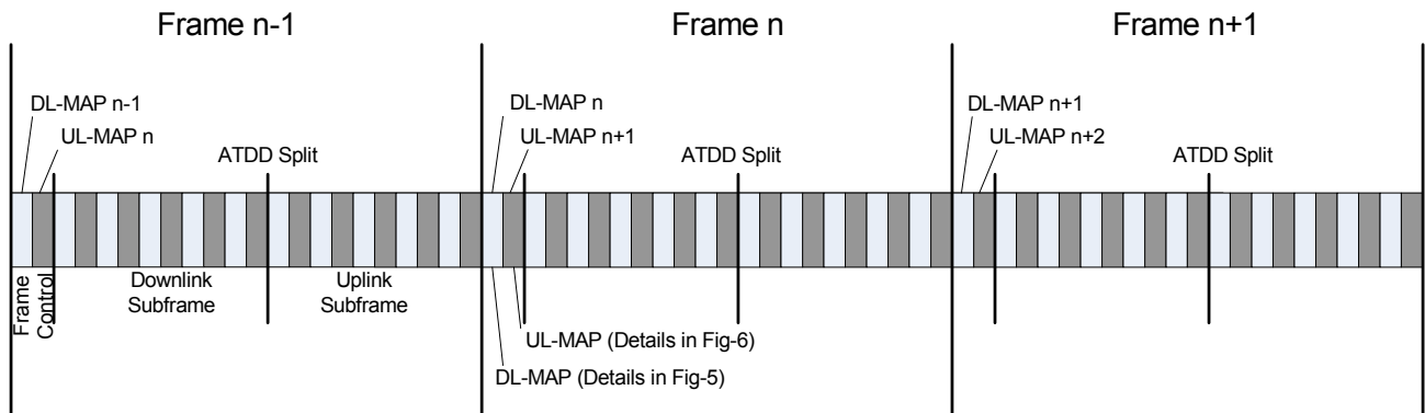
Fig (4) Time relevance of DL-MAP and UL-MAP (TDD)
